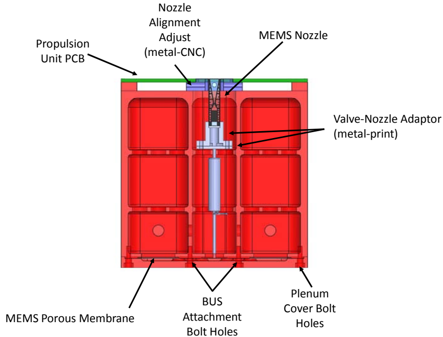
Figure 7. Cutaway Top View of Propellant Tank Showing Buried Valves, Heater and Nozzle
