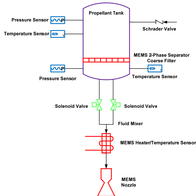
Figure 4. Schematic of the RAMPART Propulsion System
