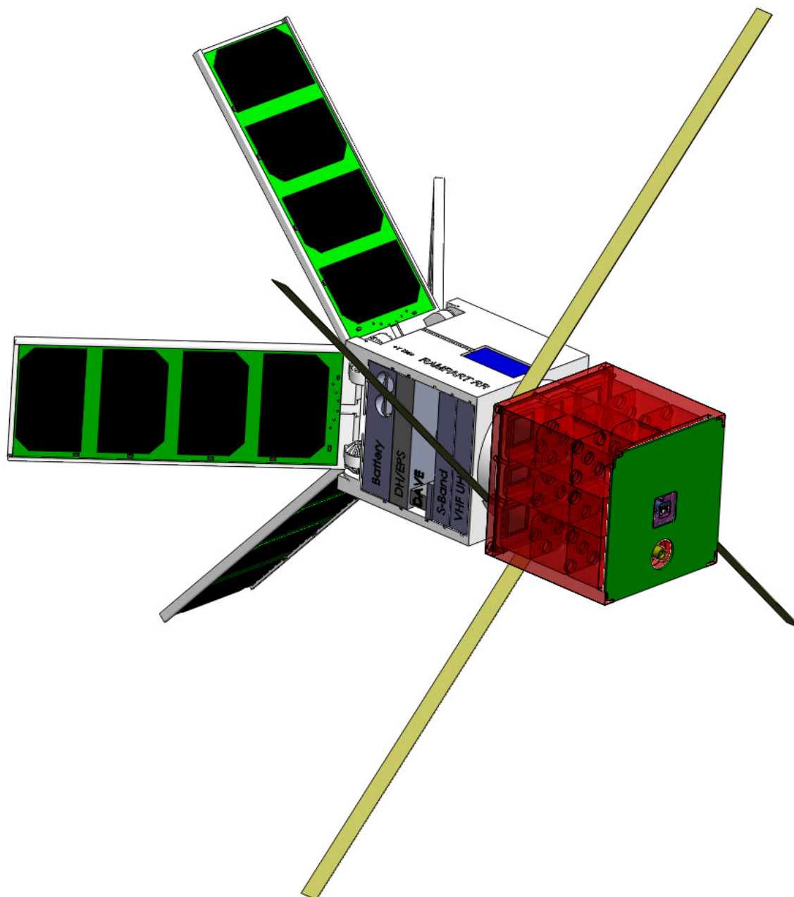
Figure 3. Deployed RAMPART 2U Cubesat with covers removed for clarity
