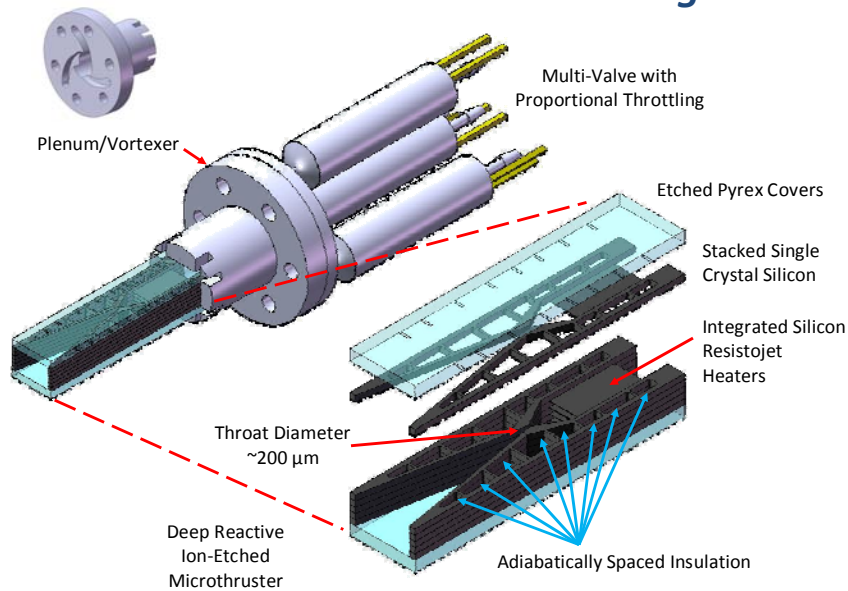
Figure 5. Enlarged View of RAMPART Thruster
