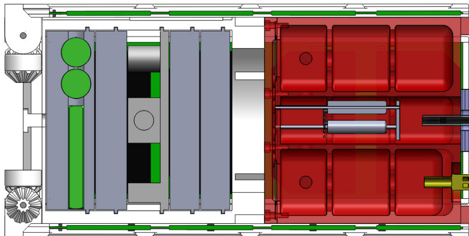
Figure 2. Cutaway View of Bus. Folded Solar Panels and Attached Propulsion Module
