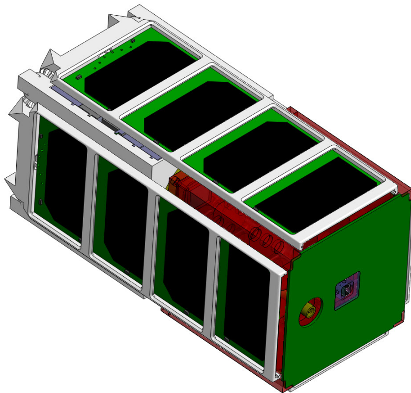
Figure 1. Stowed view of RAMPART Cubesat
