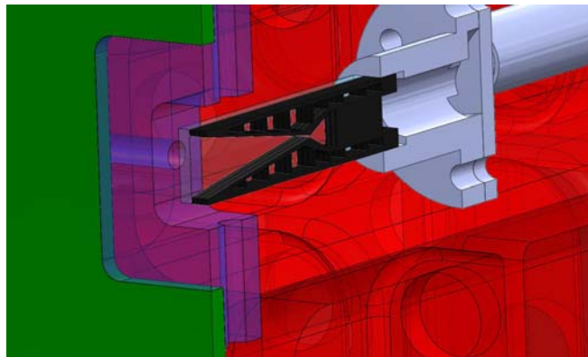
Figure 6. MEMS Heater/Nozzle Assembly
