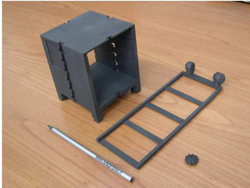
Figure 10. Laser-Printed WINDFORM RAMPART Card Cage and Solar Cell Support Panel
